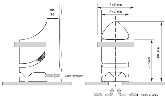
Example of installation in front of a glass or sauna wall (air supply from the side) / installation in the cabin center (air supply from below).
