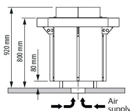
Example of installation in the cabin center (air supply from below). Installation in front of a glass or sauna wall (air supply from the side) also possible.
