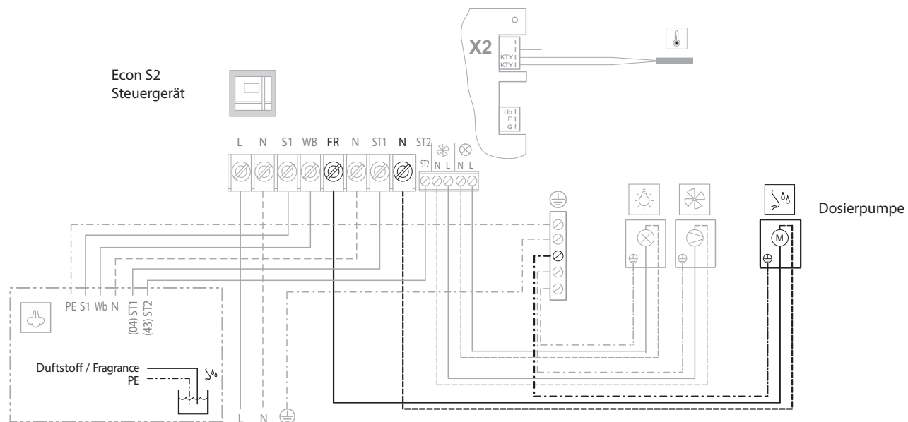
SteamRock Basic Dampfgenerator
