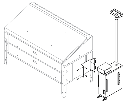
Mounting to Invisio XL
