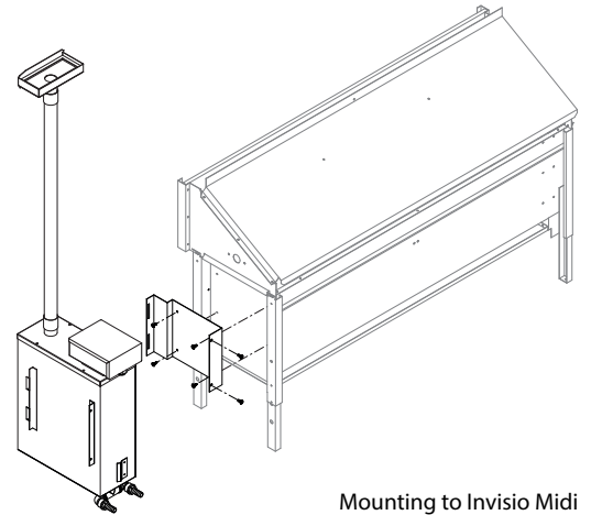
Mounting to Invisio Midi
