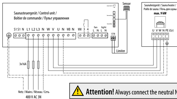
Connection example for Emotec / EmoStyle / EmoTouch control units
