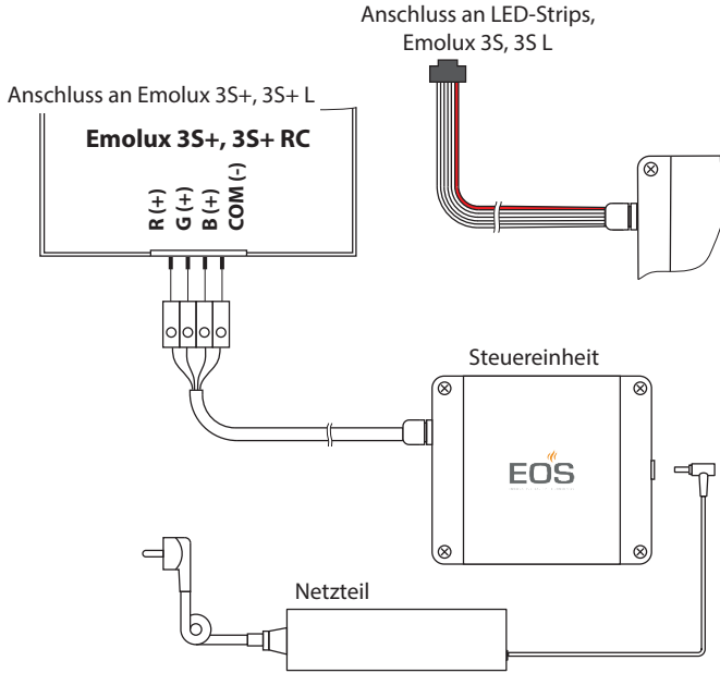
Anschluss an LED-Strips, Emolux 3S, 3S L
