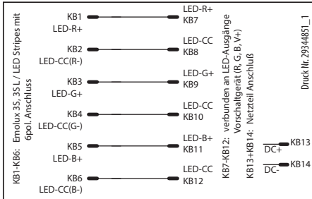
Anschluss an LED-Strips, Emolux 3S, 3S L
