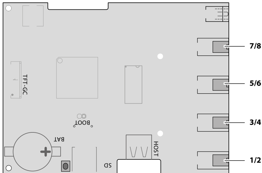
Platine EmoTouch 3 – Buchsen
