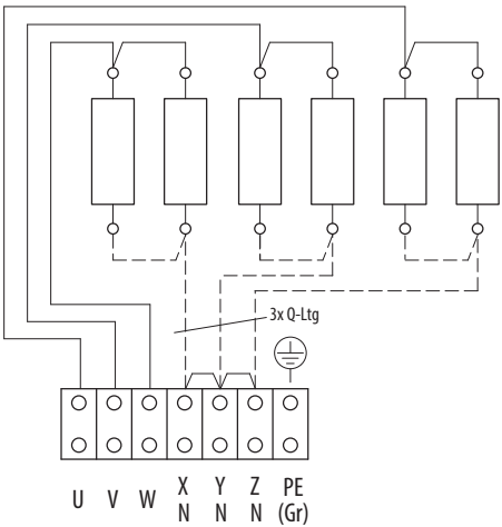
9,0 kW = 6x 1500 W
